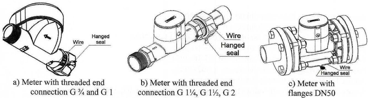
Fig. 5. Sealing of the water meter QALCOSONIC W1 after installation
